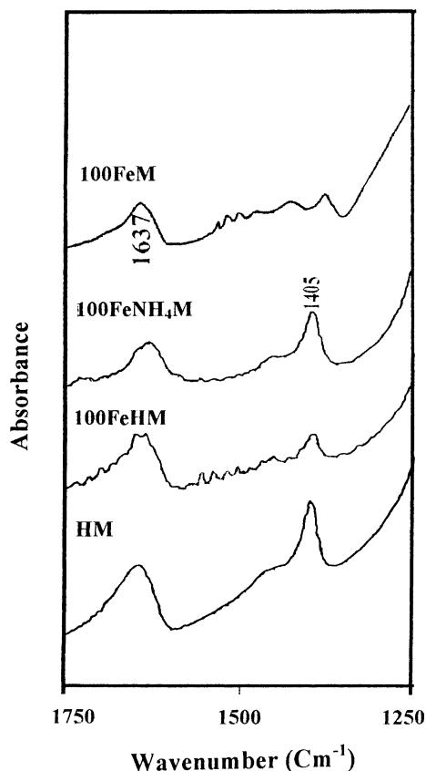
Fig. 3. IR spectra of chemisorbed ammonia on HM, 100 FeM, 100 FeHM and 100 FeNH 4 M samples.
